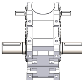
Double end solid shaft
