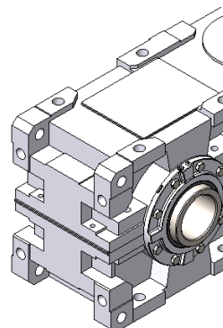
Parallel hollow shaft with keyway
